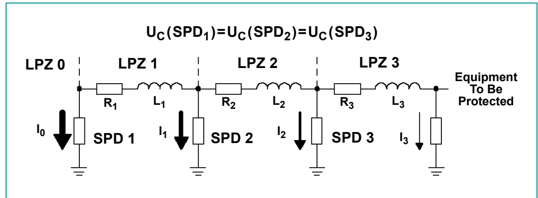
FIGURE 1. Coordination of Surge Protection Devices.
